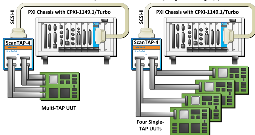
CPXI-1149.1/Turbo with ScanTAP-4 Configurations.
